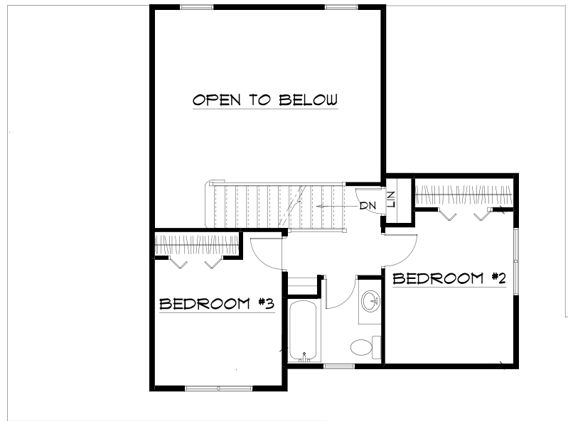
SECOND FLOOR LAYOUT
